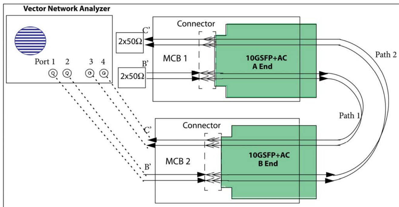
FIGURE 5 CABLE S-PARAMETERS CROSSTALK MEASUREMENT
