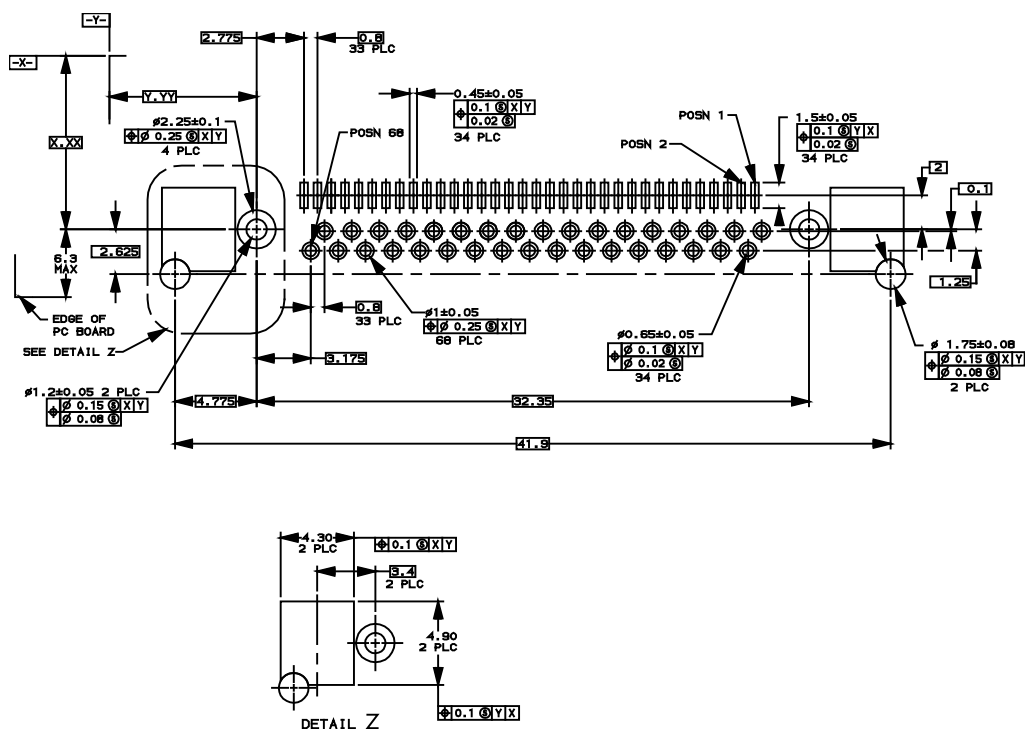
Figure 33 - Fixed board right angle hybrid
