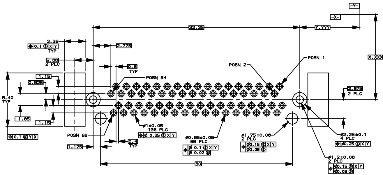
Figure 29 - Fixed board straight thru hole
