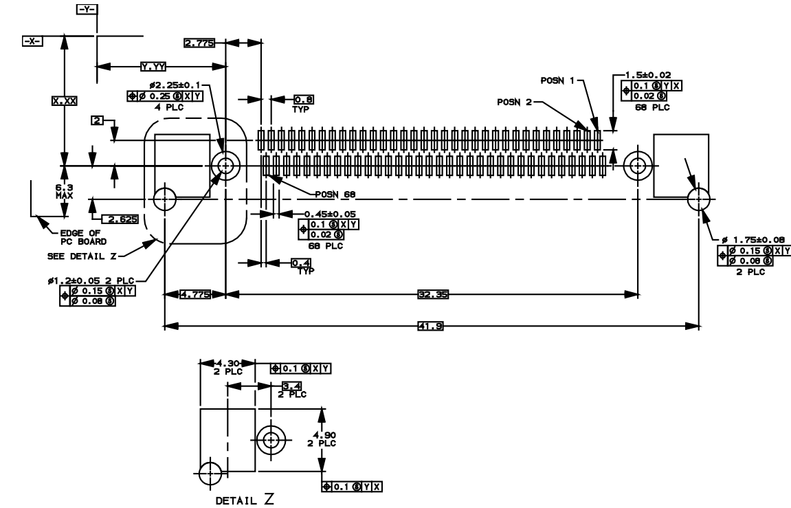
Figure 30 - Fixed board right angle surface mount dual row
