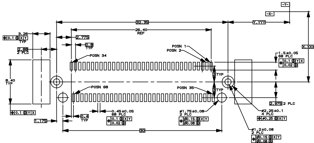
Figure 28 - Fixed board straight surface mount dual row
