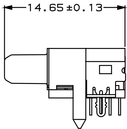
Figure 7 - Fixed board right angle outline dimensions
