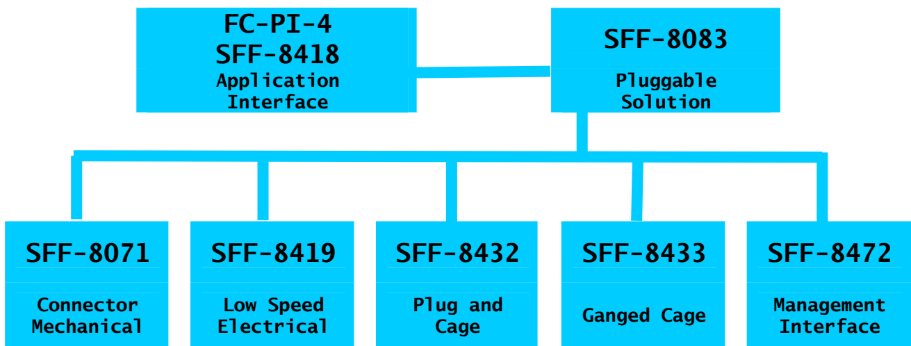
FIGURE 3-1 SPECIFICATIONS NEEDED TO IMPLEMENT A 10 GB/S PLUGGABLE TRANSCEIVER
