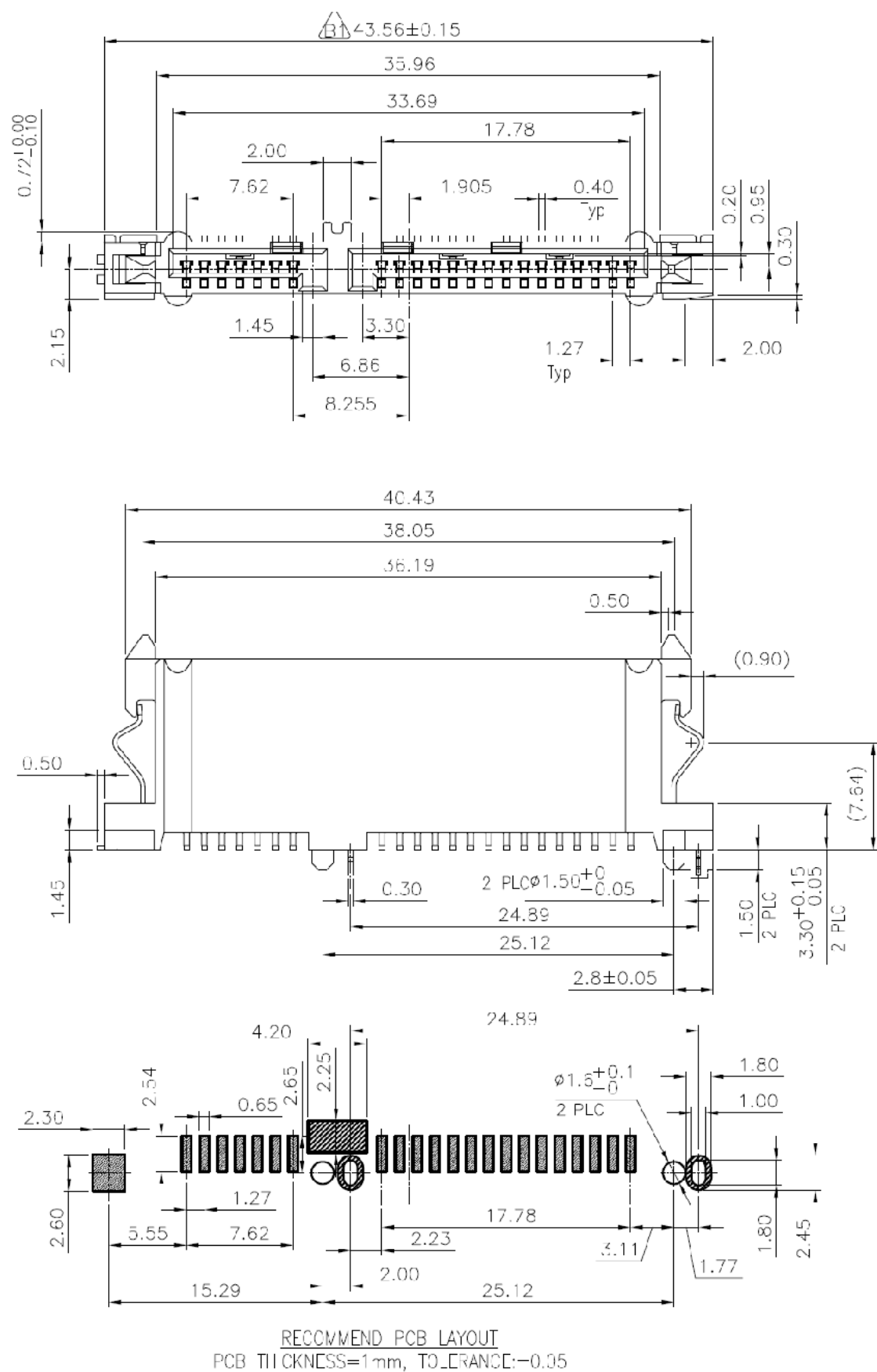
Figure 1 SATA Connector - Vertical Mount
