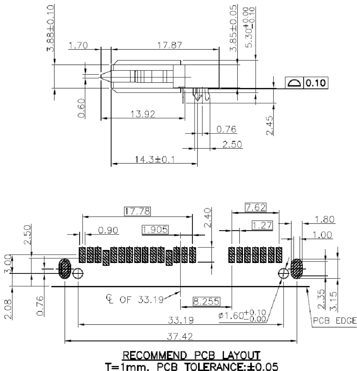
Figure 3 SATA Connector - Horizontal Mount (2 of 2)
