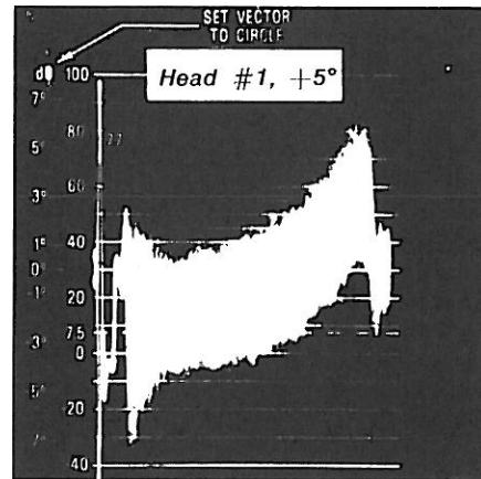
Figure 14. Differential Phase
