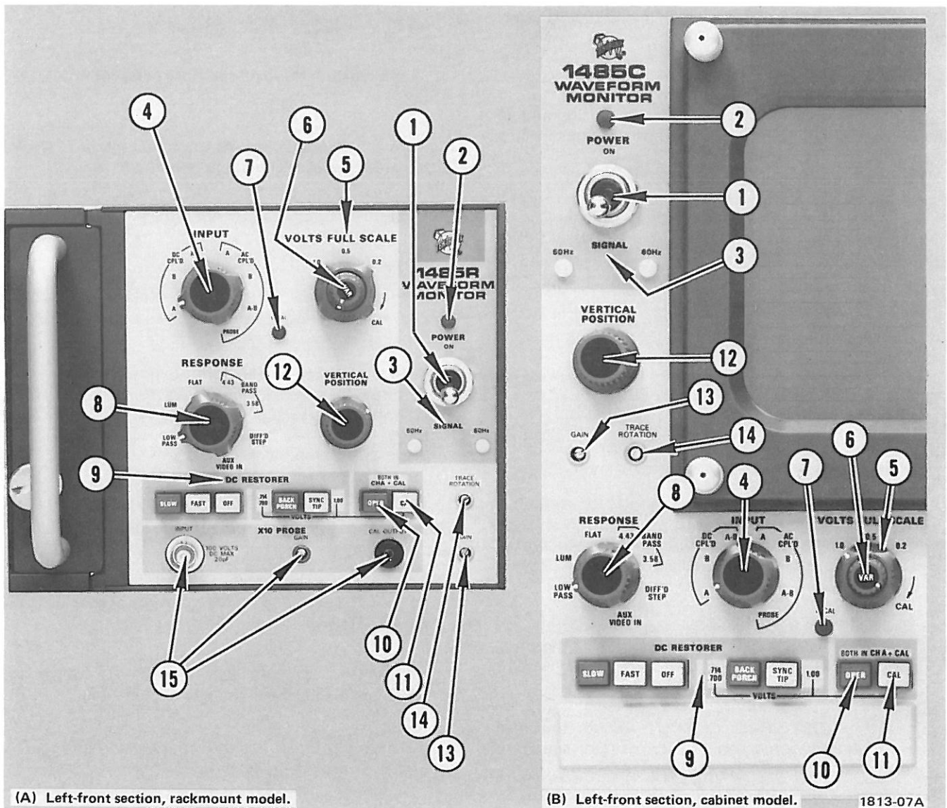
Fig. 2-1. Vertical control locations for rackmount, left, and cabinet model, right.
