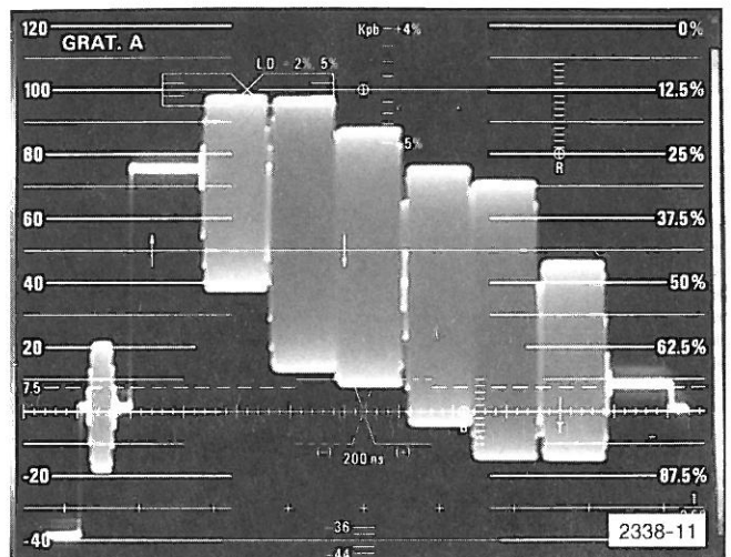
Fig. 1-12. A one-line display of a test signal at 5 \mu S/Division.
