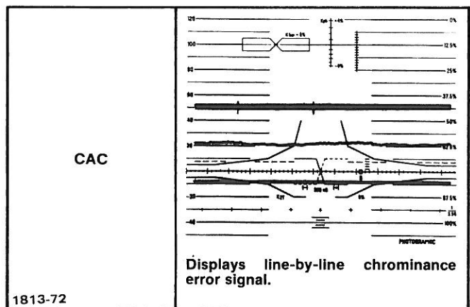
Fig. 2-11. TR70C operating waveforms (cont).
