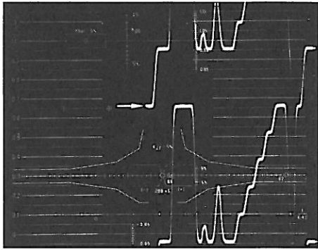
Figure 5c. As Figure 5a but LOWPASS response.
