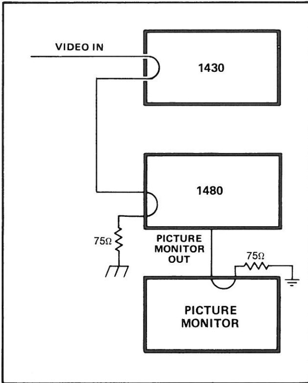
Figure 6. Equipment connections for head-by-head noise measurement.
