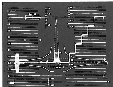
Figure 1. Measurement of K_{hor} and K_{ph} .
