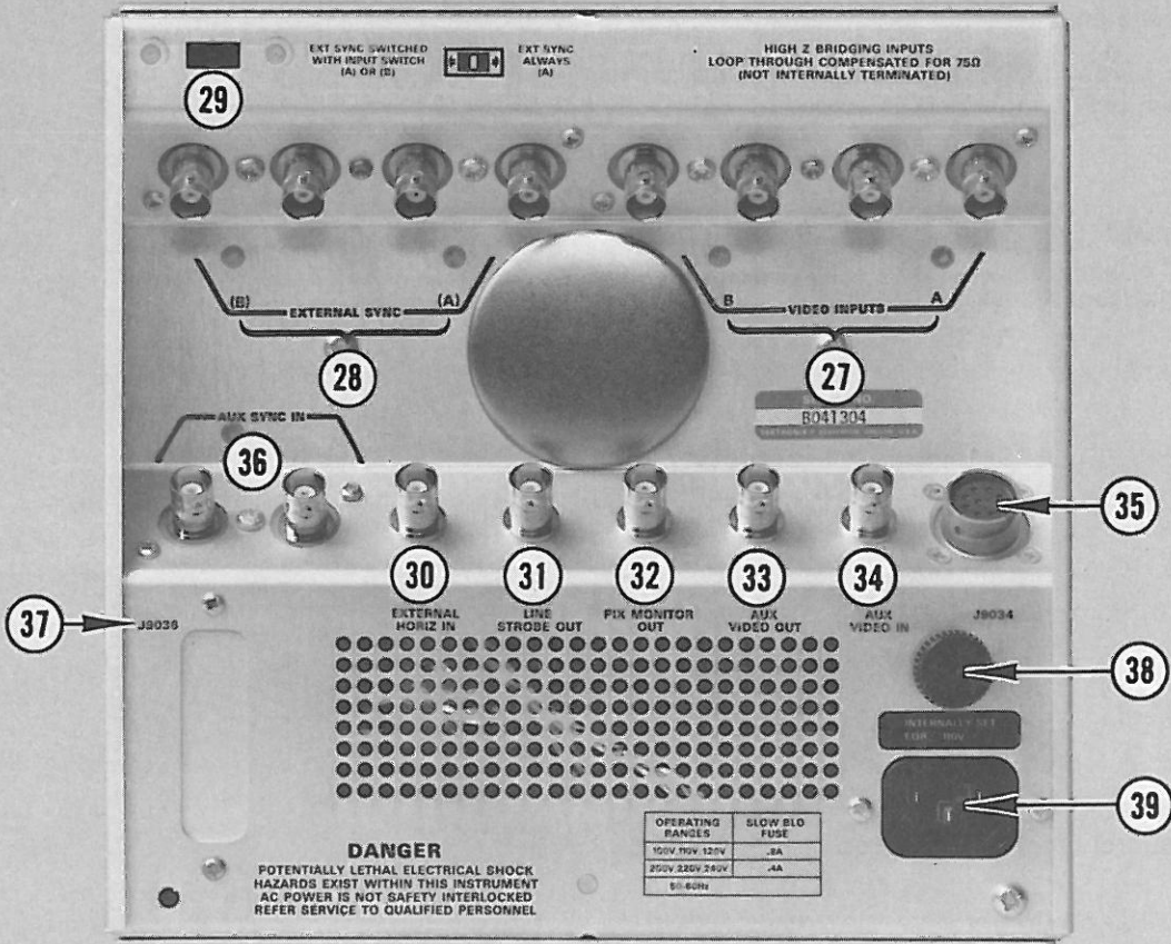
(A) Rackmount model rear panel.
