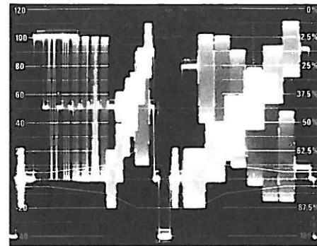
Figure 1. Two VITS lines from each field.
