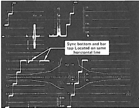
Figure 3a. Correct setting with gain normal.
