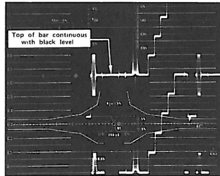
Figure 7a. Measurement of picture component, level correct.
