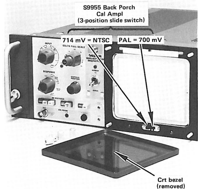
Fig. 2-7. Location of the Back Porch Cal Ampl switch, S9955. Same location for both rackmount and cabinet model.
