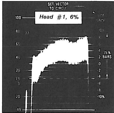
Figure 13. Differential Gain
