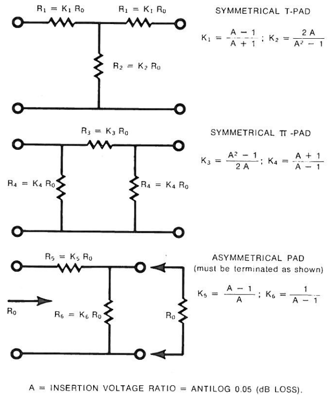
Figure 5. Design of Attenuator Pads.
