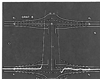
Figure 5. K_{2T} measurement with increased gain, K_{2T} > 1\% .
