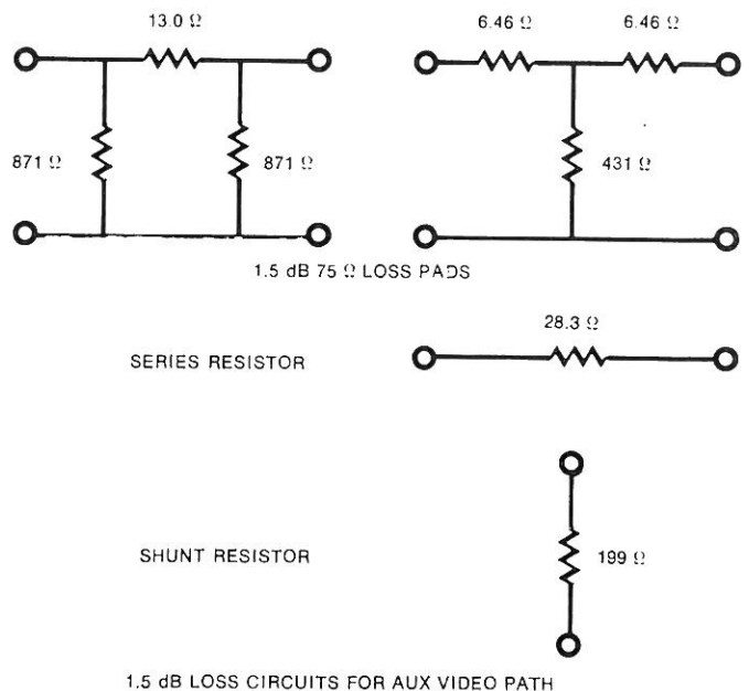
1.5 dB LOSS CIRCUITS FOR AUX VIDEO PATH
