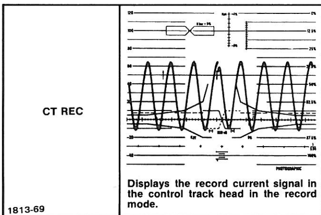
Fig. 2-11. TR70C operating waveforms (cont).
