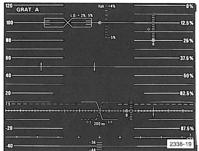
Fig. 2-5. NTSC Composite Graticule A supplied with 1480 and 1485.
