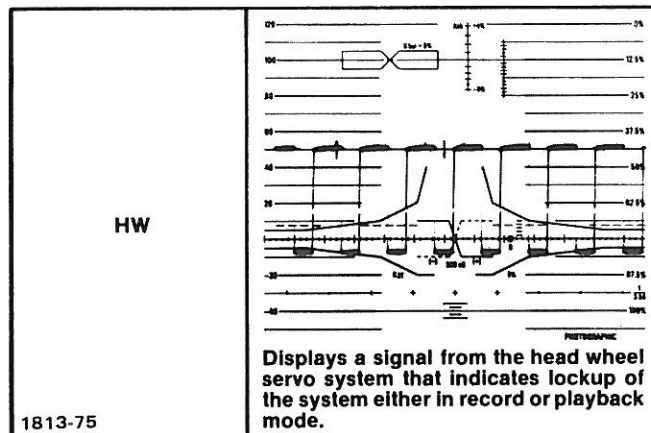
Fig. 2-12. TR70C operating waveforms (cont).
