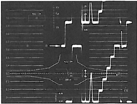
Figure 5b. As Figure 5a but IRE response.
