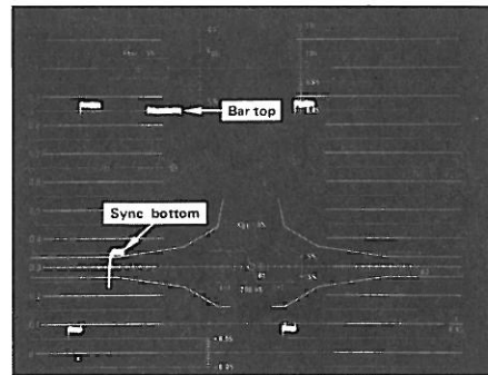
Figure 4. Level 10% high, X 5 gain.
