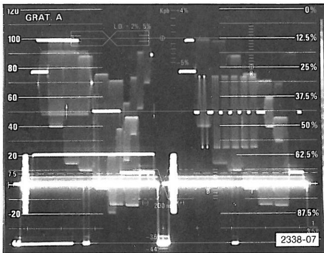
Fig. 1-8. 15-Line display with both active and vertical interval lines.
