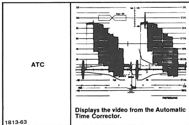
Fig. 2-10. Operating waveforms from RCA Video Tape Recorder model TR70C.
