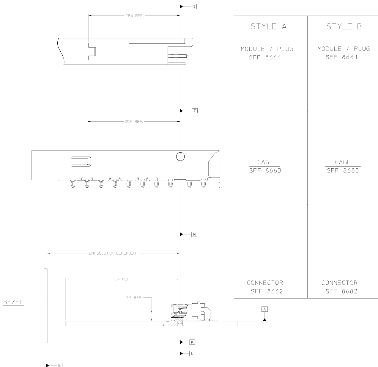
FIGURE 4-1 DATUM DEFINITIONS
