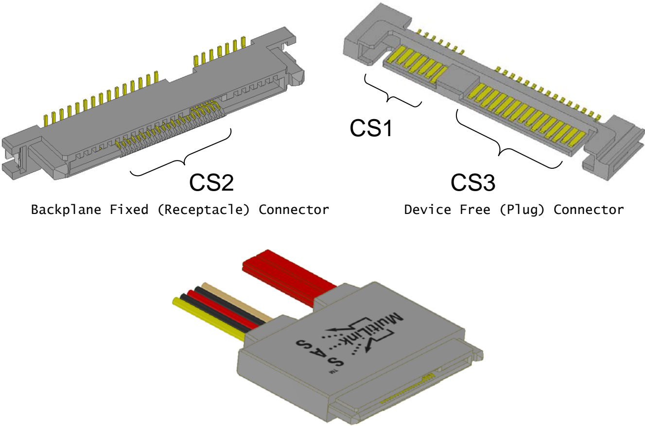
Cable Fixed (Receptacle) Connector FIGURE 4-1 GENERAL VIEW CONNECTORS AND DESCRIPTIONS
