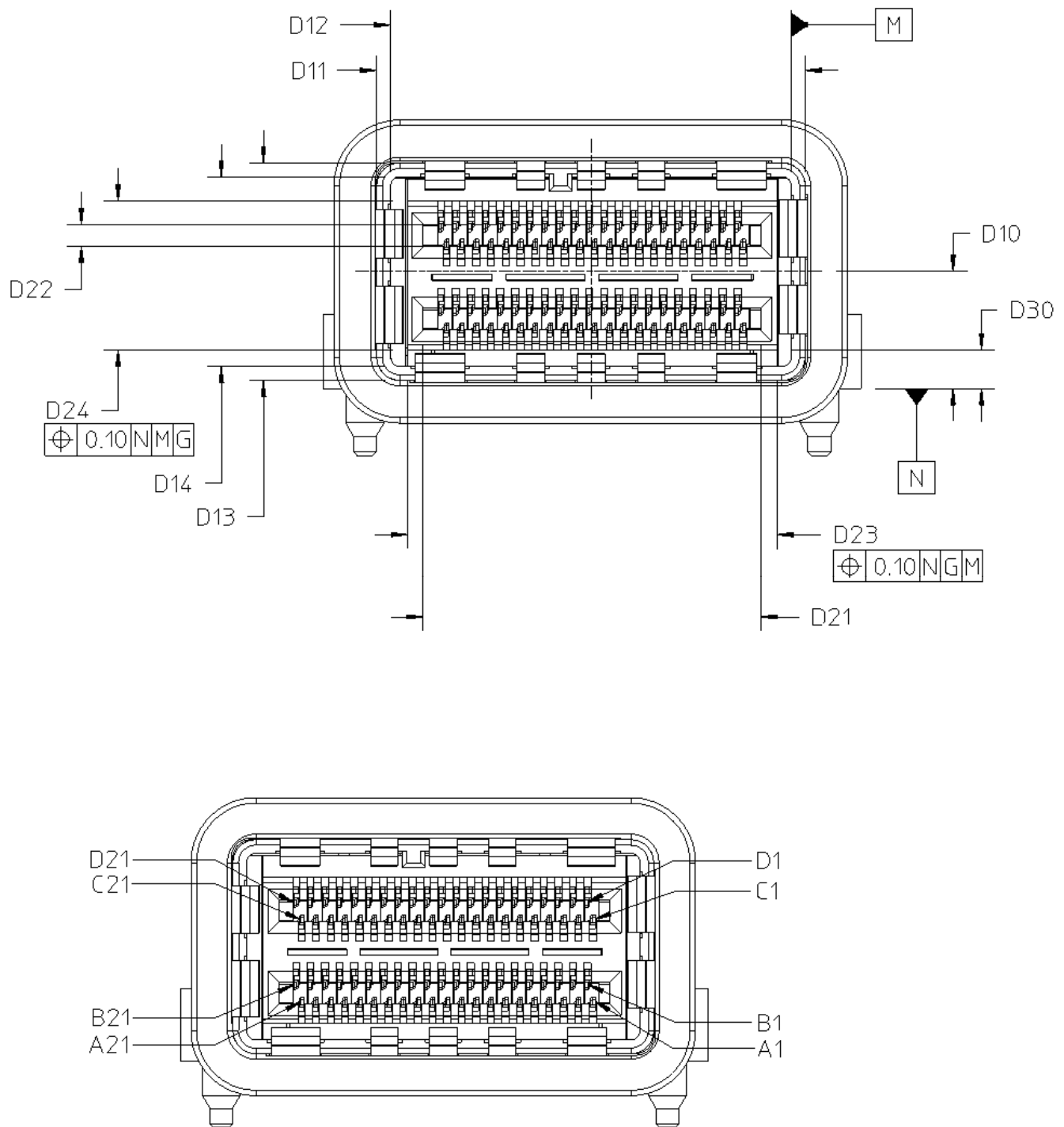
FIGURE 5-8 RECEPTACLE (2)
