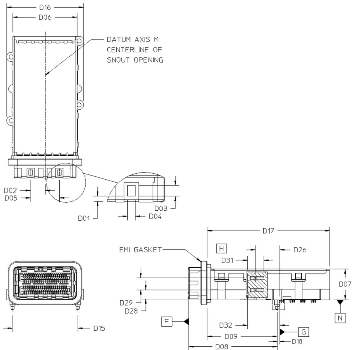
FIGURE 5-7 RECEPTACLE (1)
