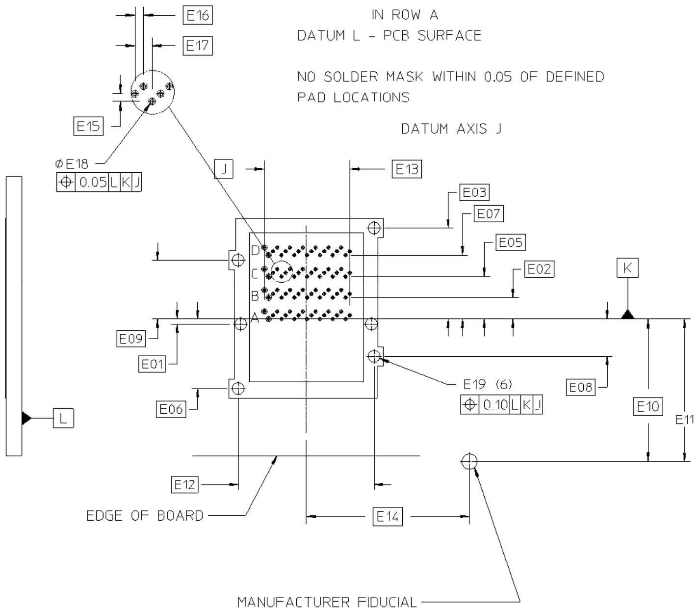
FIGURE 5-10 RECEPTACLE FOOTPRINT
