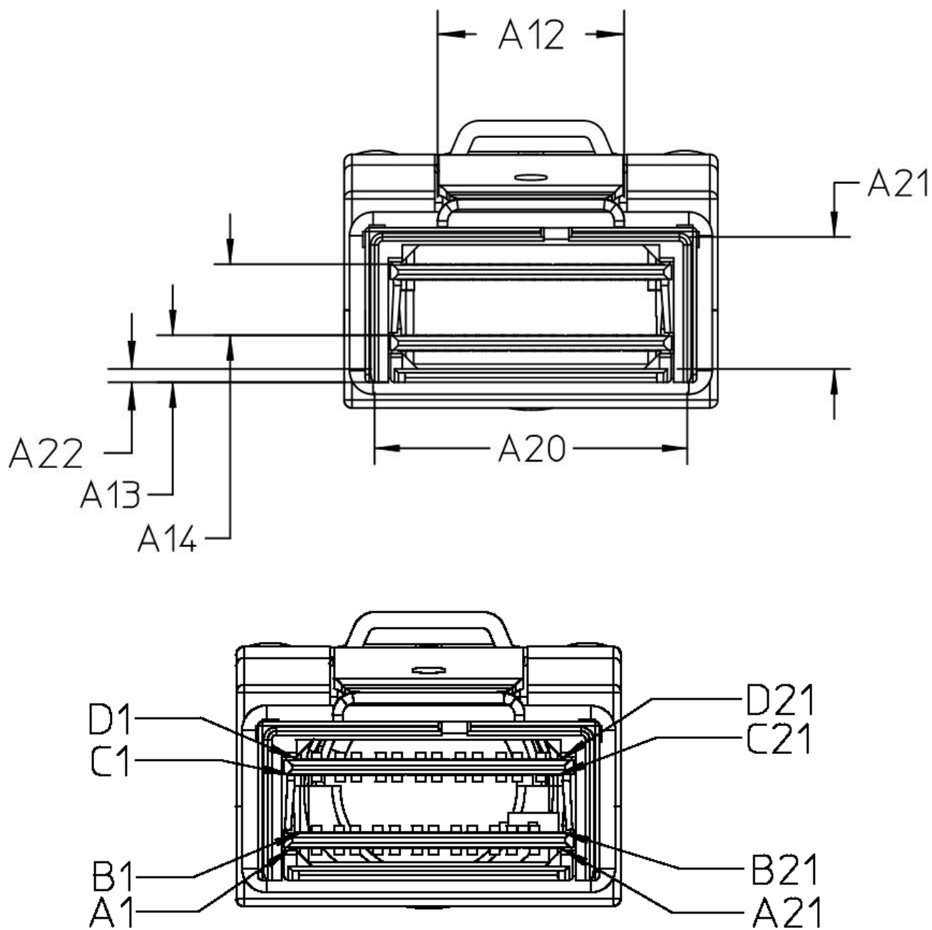
FIGURE 5-4 PLUG (3)
