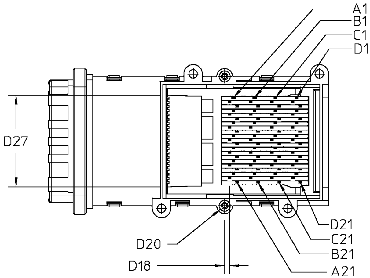
FIGURE 5-9 RECEPTACLE (3)
