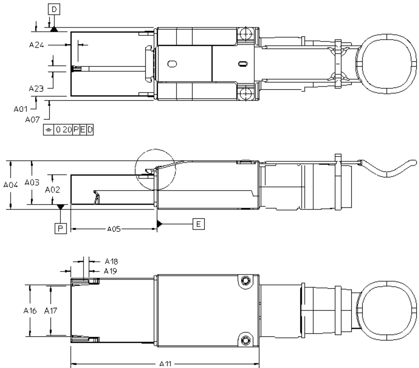
FIGURE 5-3 PLUG (2)
