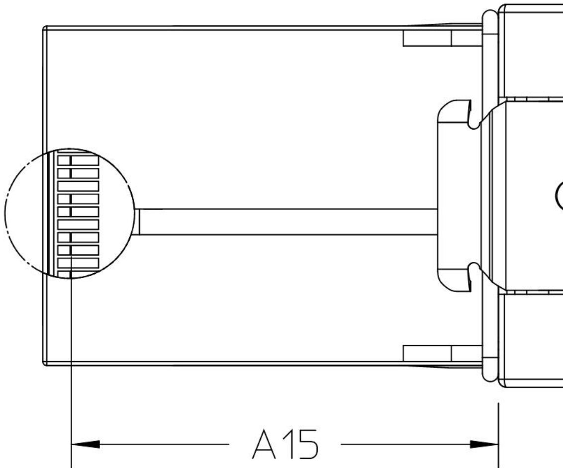
FIGURE 5-2 PLUG (1)
