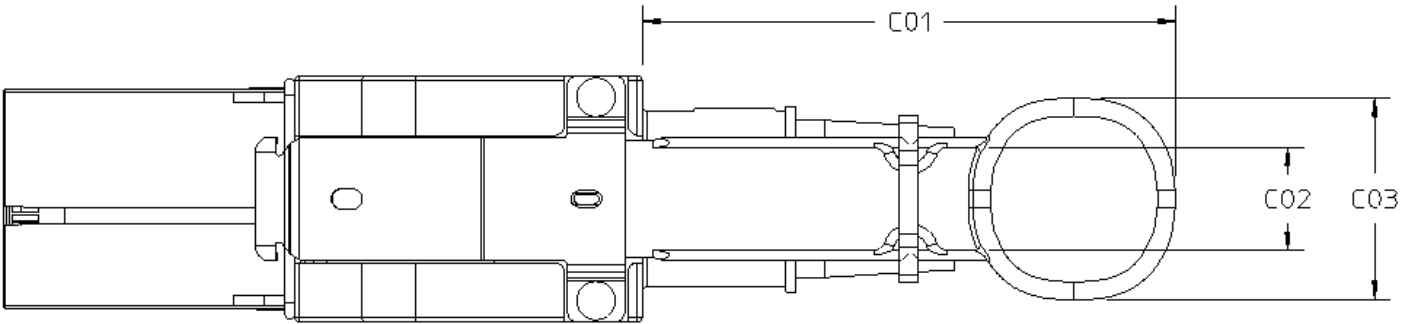
This is one possible configuration, color may be specified by the application. FIGURE 5-6 PLUG PULL TAB EXAMPLE
