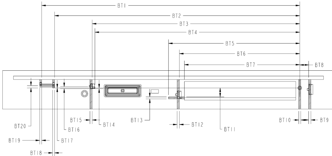
Figure 8.18 Areas where ribs shall be implemented in a cored bezel
