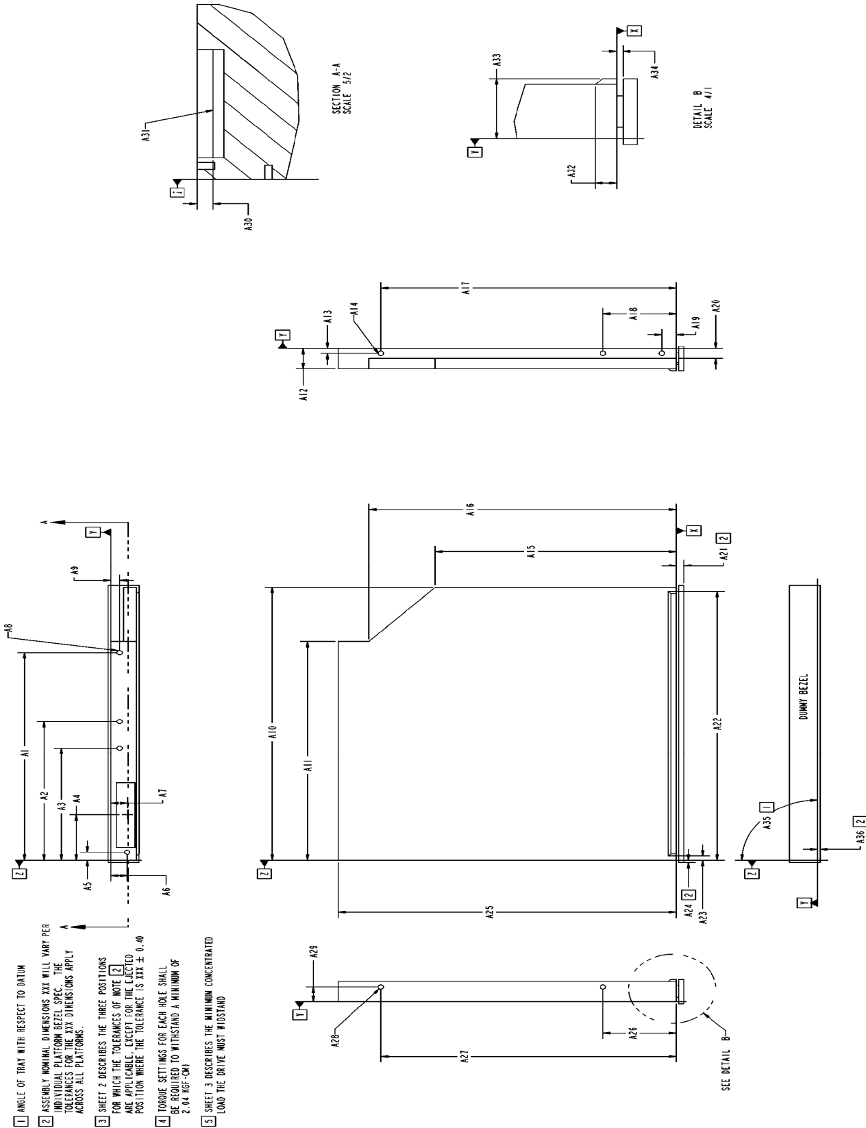
Figure 5-1: Sheet 1 - 5 1/4" 9.5mm Height Optical Drive Parallel ATA Form Factor
