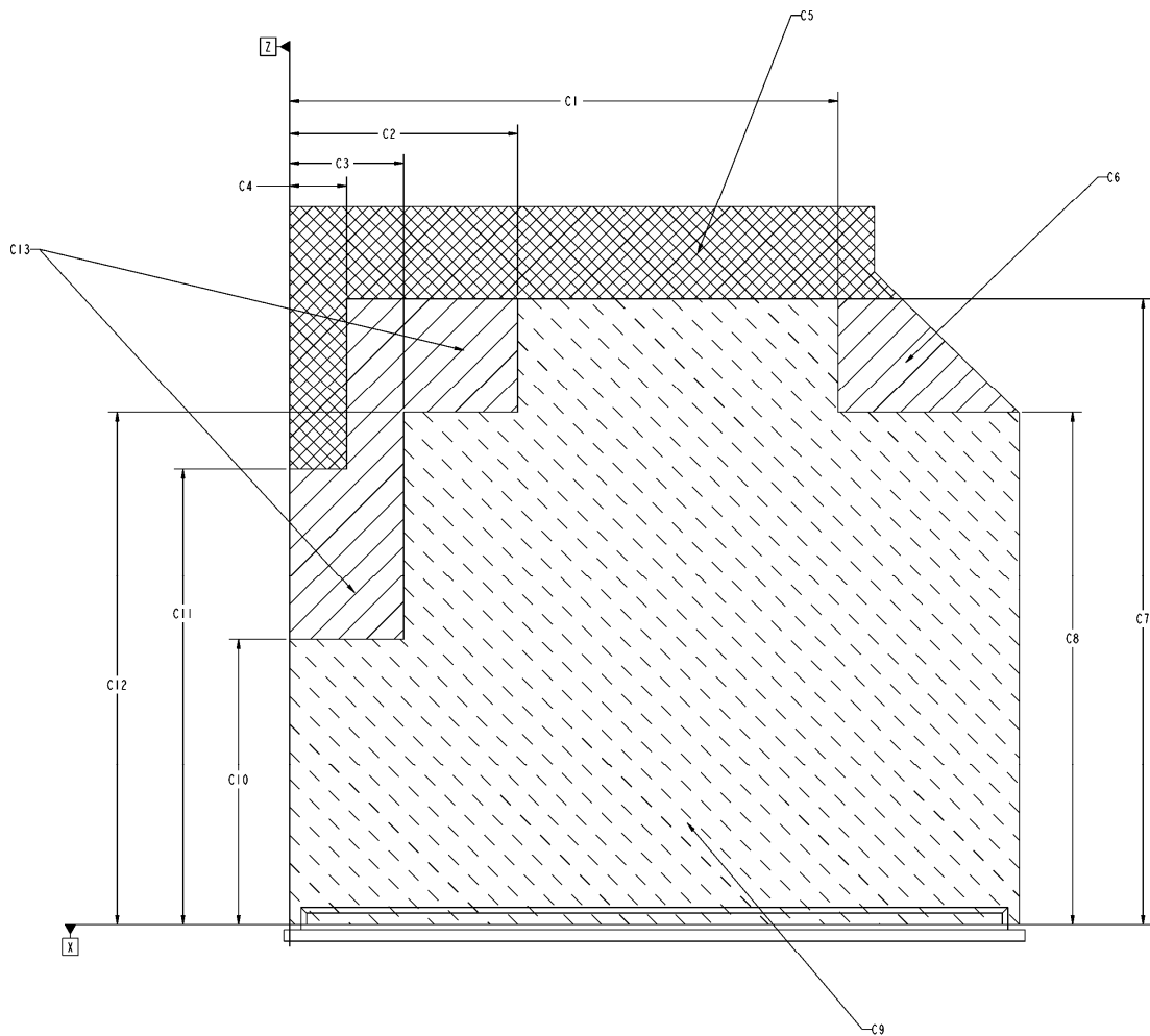
Figure 5-2: Sheet 2 - Tray Positions
