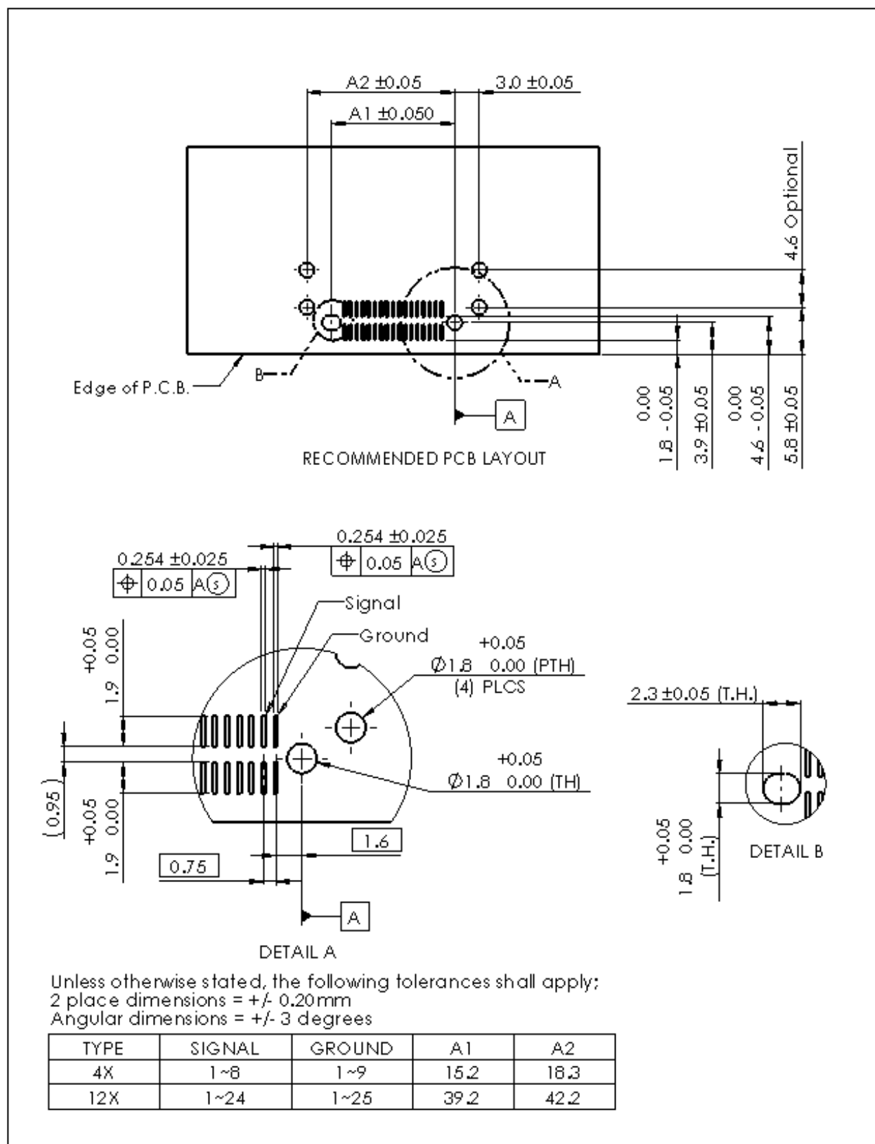
Figure 3 - Fixed board 2 row ST footprint
