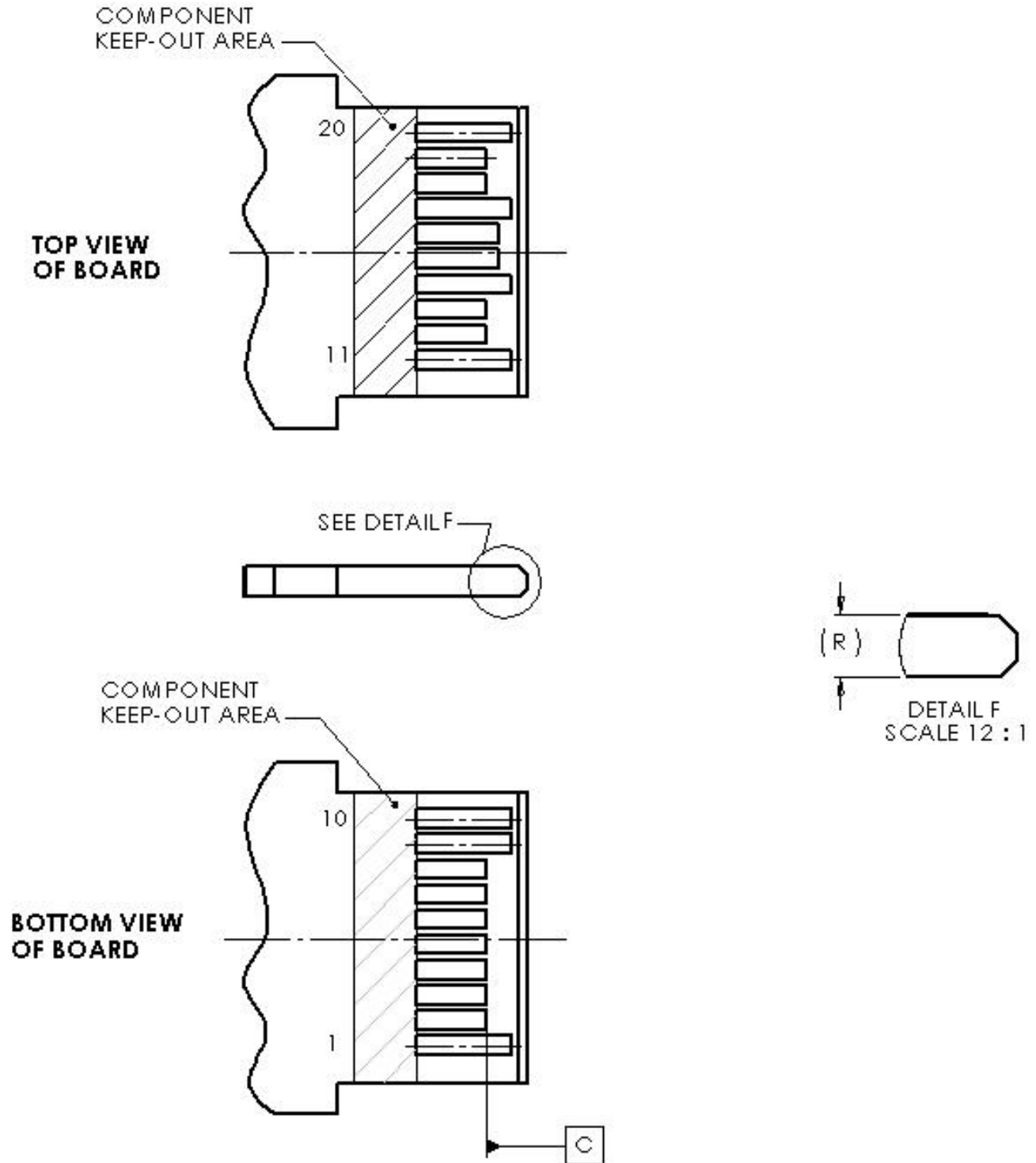
FIGURE 4-3: MODULE ELECTRICAL INTERFACE
