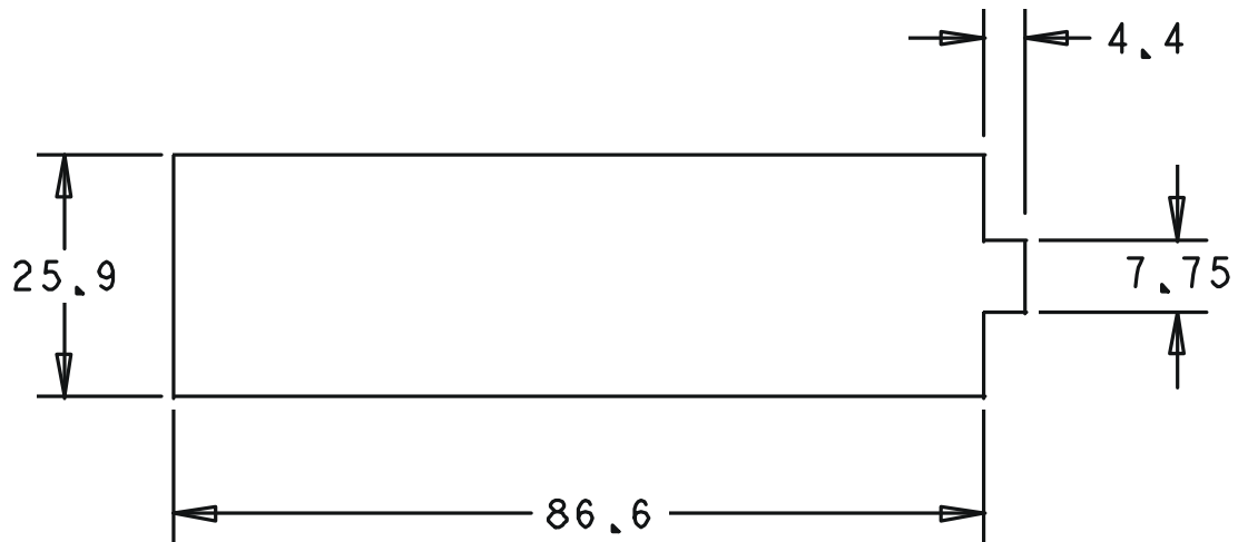
Figure 16 - Panel cut out for 6 position patch panel receptacle
