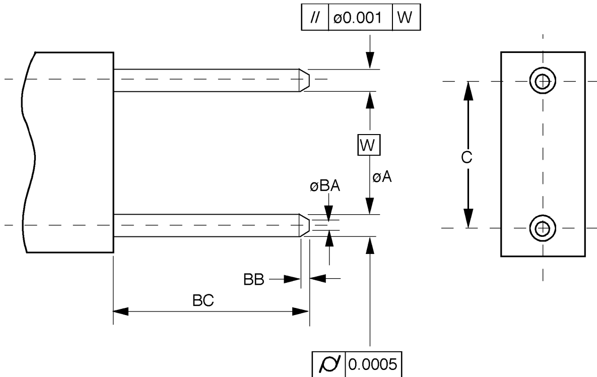
Figure 21 - Guide hole gauge assembly
