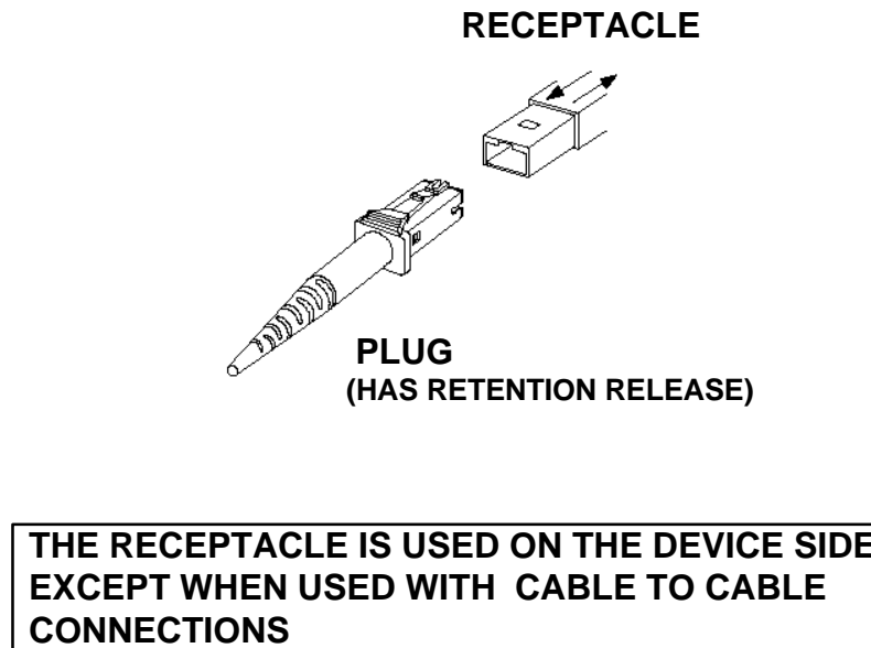
Figure 4 - Mating side housing gender definitions
