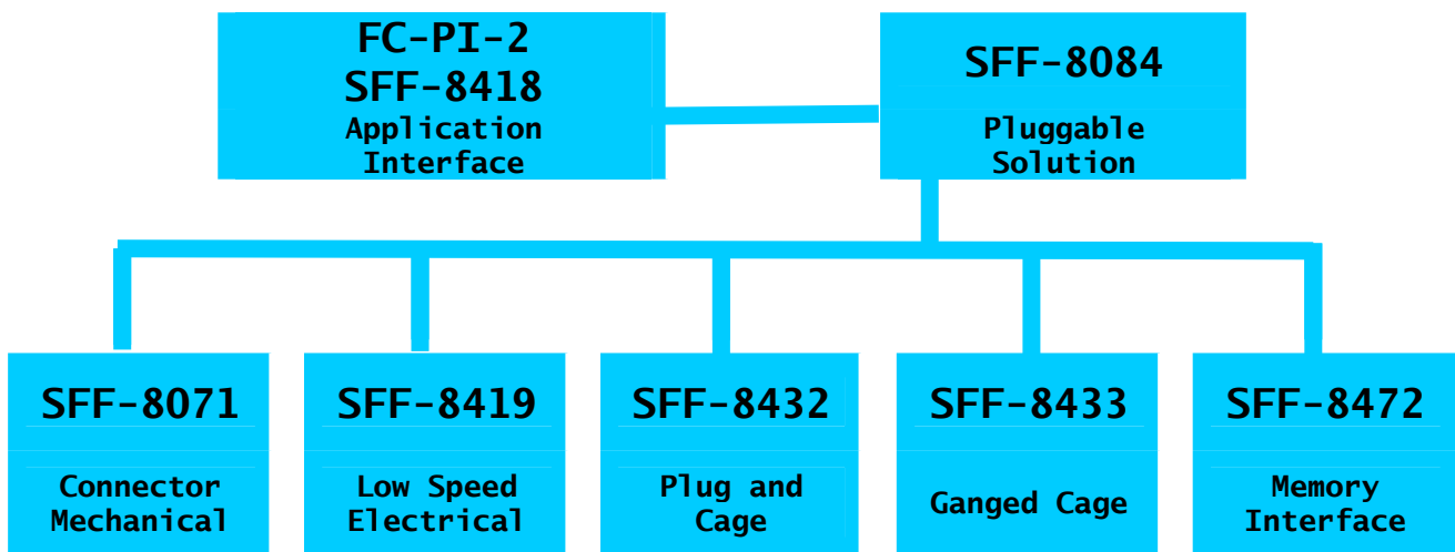
FIGURE 3-1 SPECIFICATIONS NEEDED TO IMPLEMENT A 4 GB/S PLUGGABLE TRANSCEIVER
